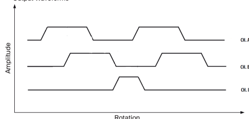
Output Waveforms
