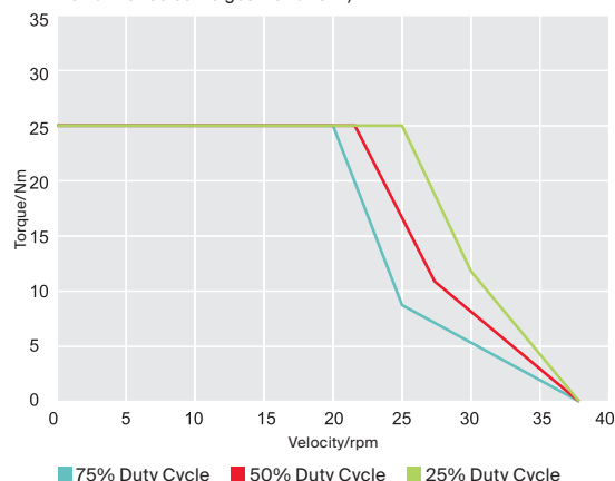
Performance curve gear ratio 101:1)
