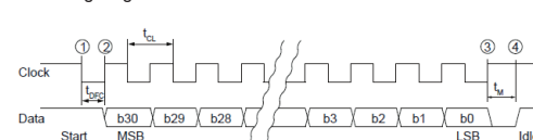
SSI timing diagram
