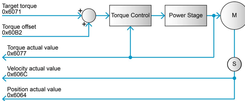
Figure 3-31 Cyclic Synchronous Torque Mode – Overview
