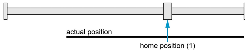
Figure 3-22 Homing method 37
