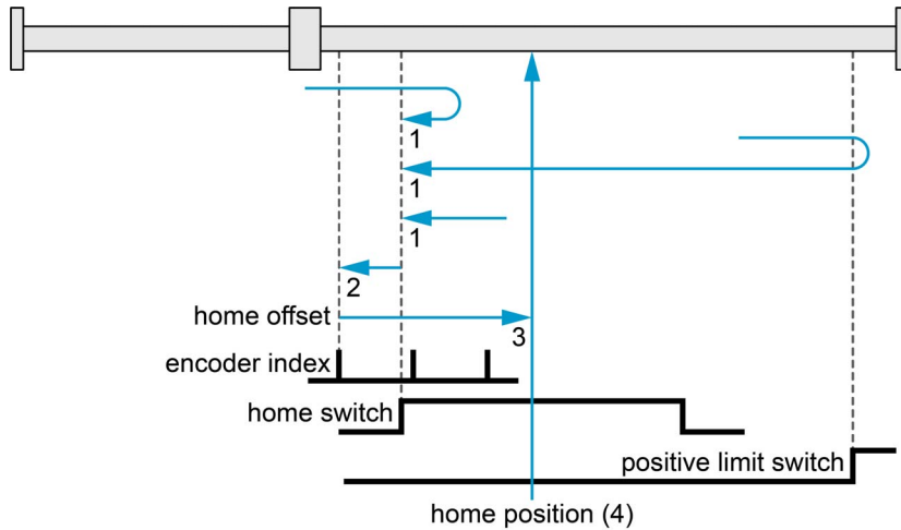
Figure 3-14 Homing method 7
