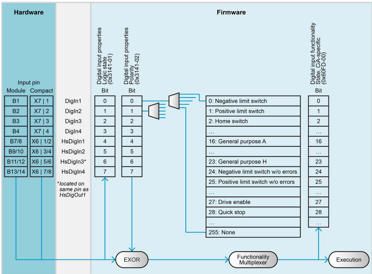
Figure 4-38 Digital input functionality
