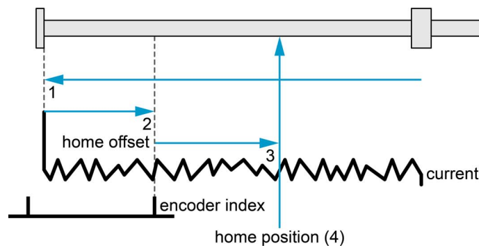
Figure 3-24 Homing method -2
