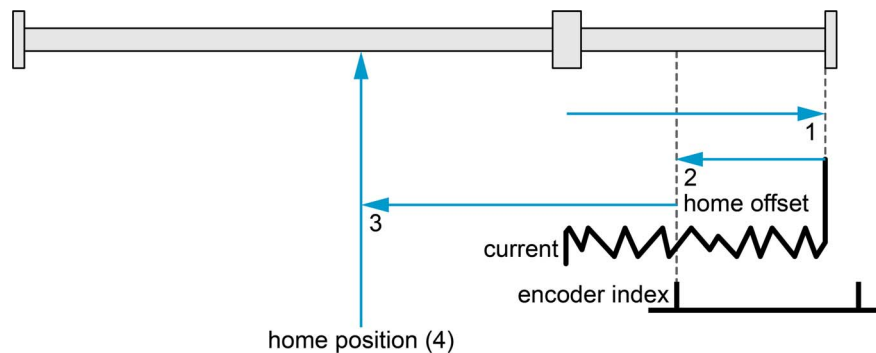
Figure 3-23 Homing method -1
