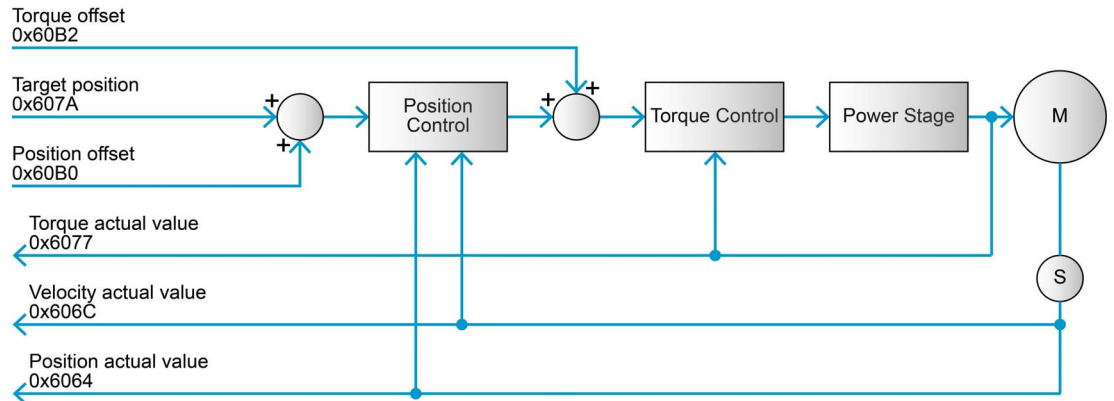
Figure 3-27 Cyclic Synchronous Position Mode – Overview
