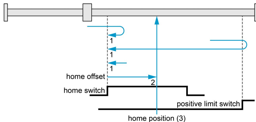
Figure 3-18 Homing method 23
