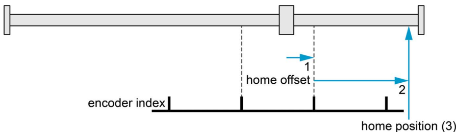
Figure 3-21 Homing method 34
