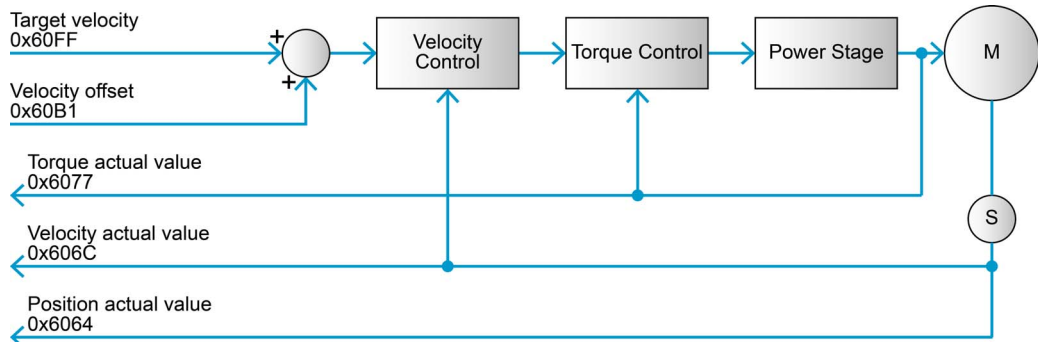
Figure 3-29 Cyclic Synchronous Velocity Mode – Overview
