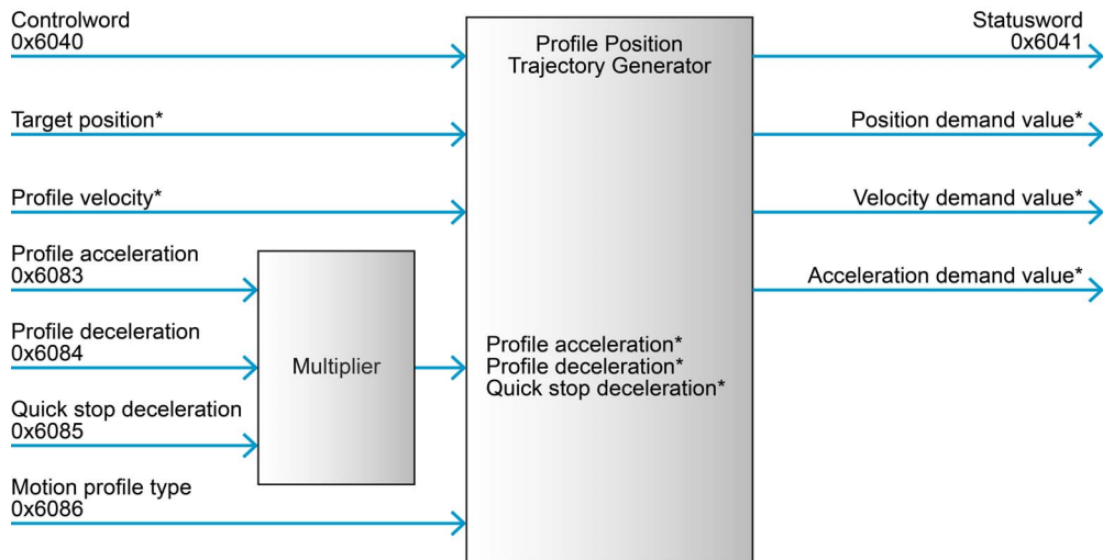
Figure 3-5 Profile Position Mode – Block diagram
