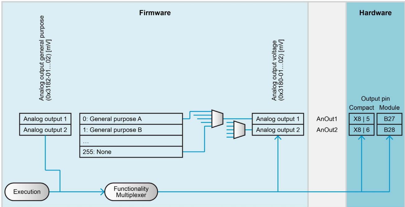
Figure 4-40 Analog output functionality
