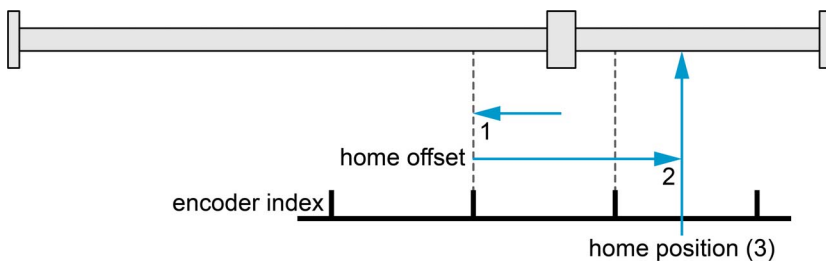
Figure 3-20 Homing method 33
