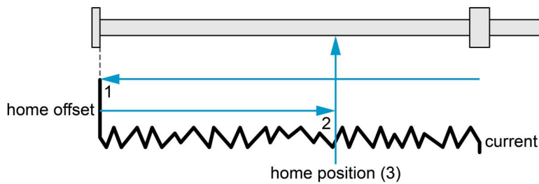
Figure 3-26 Homing method -4
