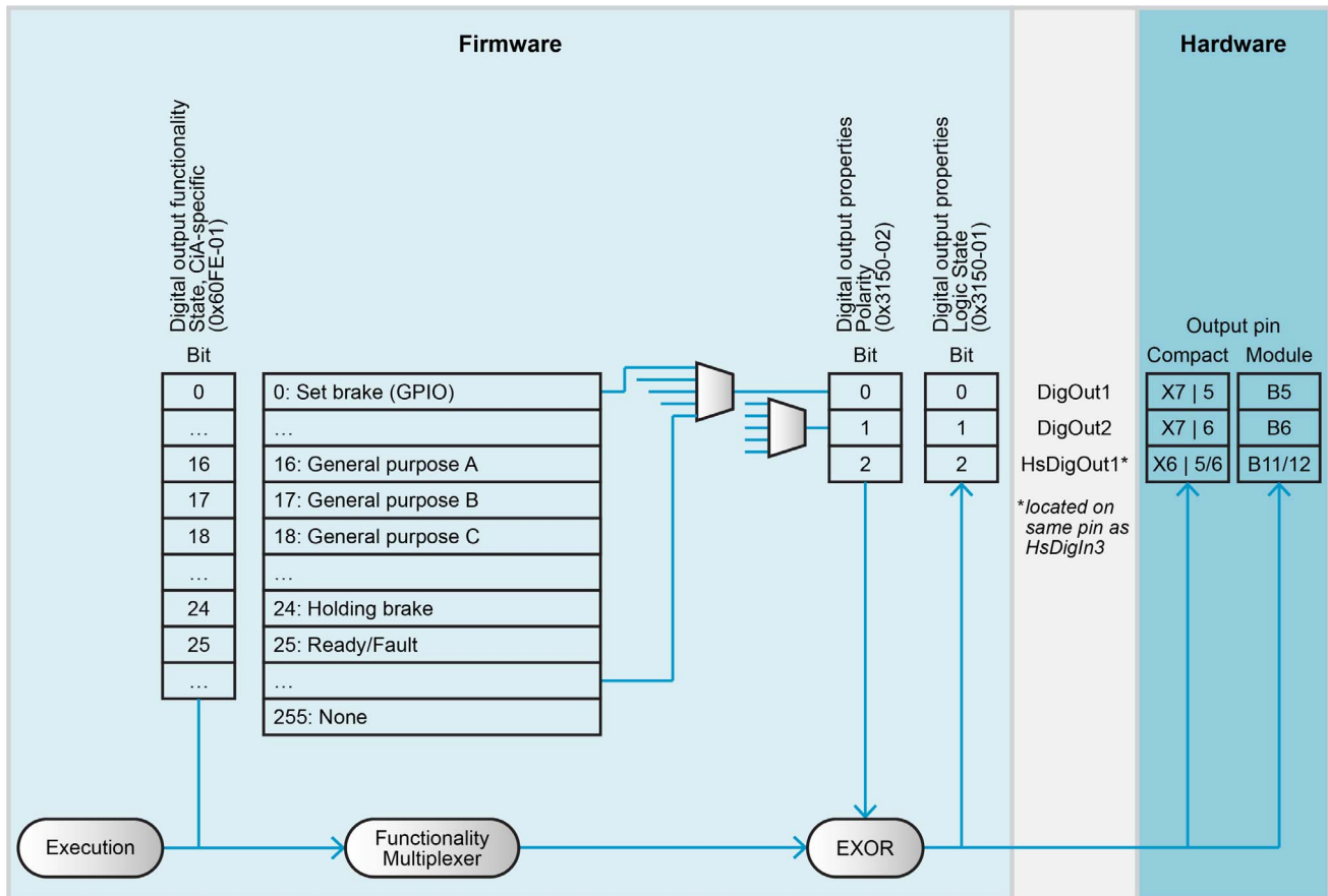
Figure 4-39 Digital output functionality
