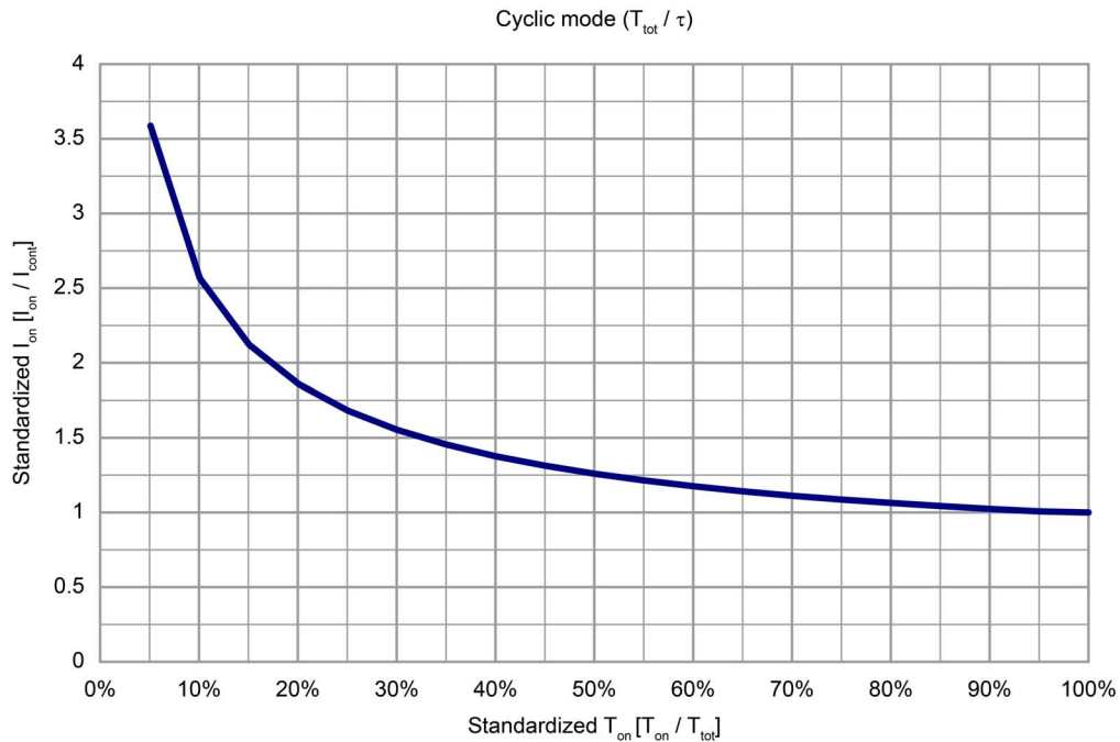
Figure 3-37 Cyclic mode standardized vs. standardized “ON time”
