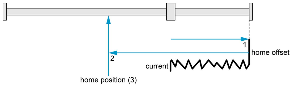
Figure 3-25 Homing method -3
