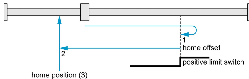
Figure 3-17 Homing method 18
