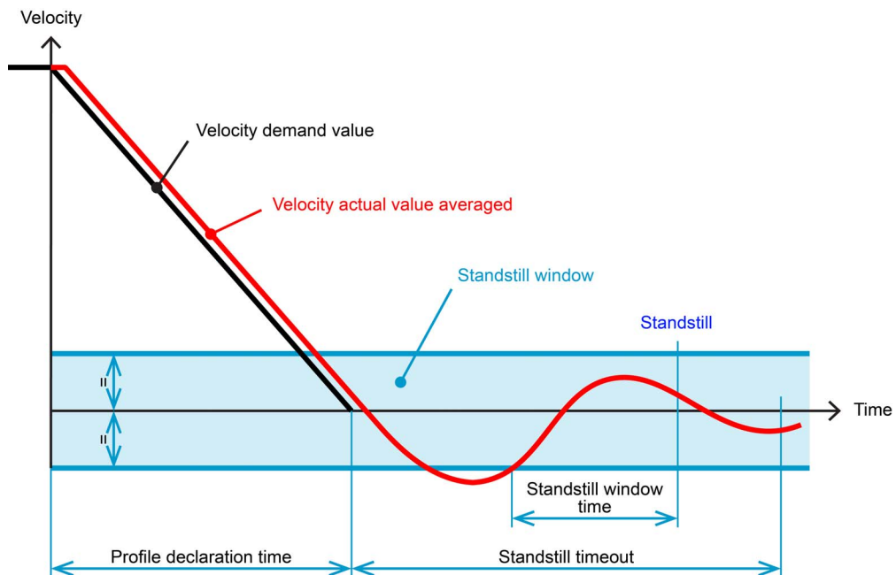
Figure 6-45 Standstill window
