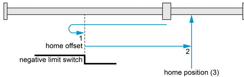
Figure 3-16 Homing method 17
