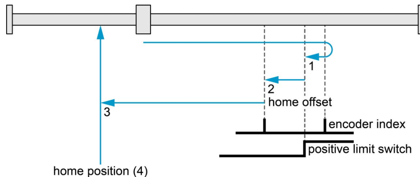
Figure 3-13 Homing method 2
