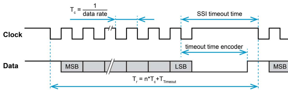
Figure 6-43 SSI encoder – Timing
