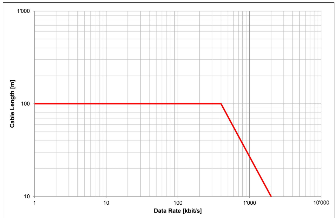
Figure 6-41 SSI encoder – Data rate vs. cable length
