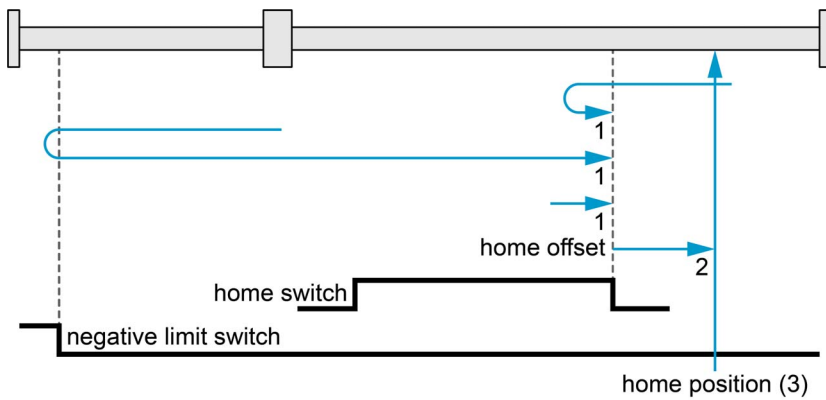
Figure 3-19 Homing method 27
