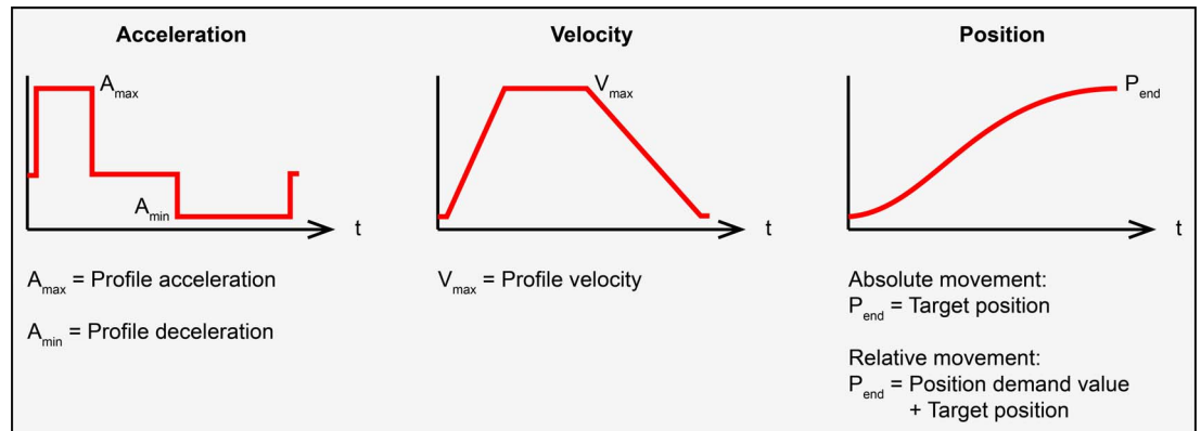
Figure 3-6 Profile position trajectory
